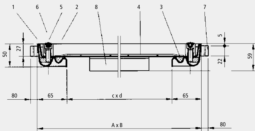
Type BV-shallow steel/BVE-shallow steel, scale 1 : 5
